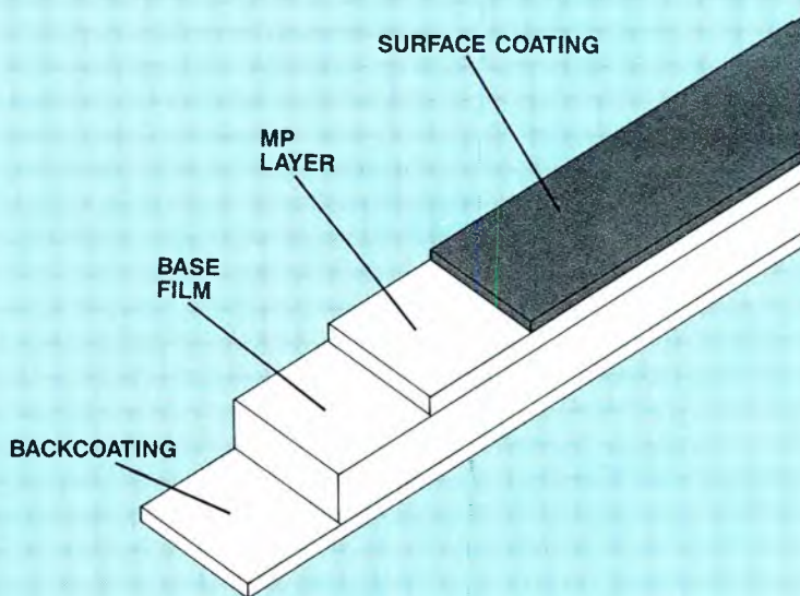
Figure 1. A cutaway view of DAT magnetic media. (MP = metal particle.)
