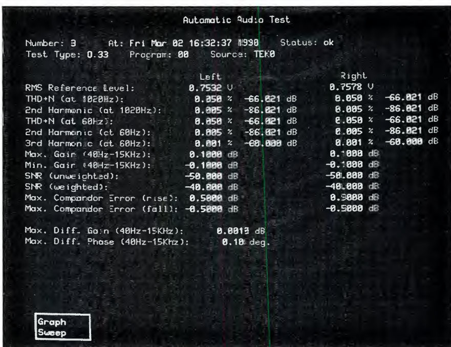
Figure 1. Display of automated audio test results for stereophonic pairs measured according to CCITT Recommendation 0.33.
