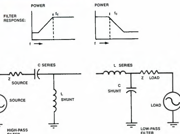
Figure 3. A bandpass filter consists of a high-pass and low-pass filter in series.
