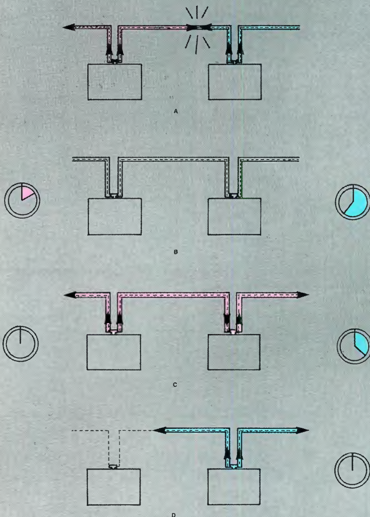
Figure 1. When users compete for the bus in a carrier-sense, multiple access with collision detection (CSMA/CD) system, it results in data collisions (a). To avoid data contamination, both users abandon the message, and back off for a random interval (b). Message packets are then retransmitted (c,d). If secondary collisions occur, the process is repeated.
