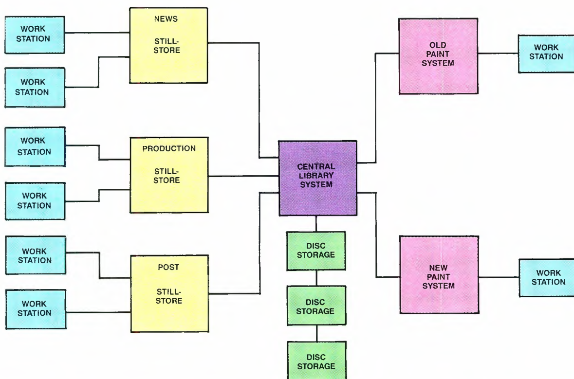
Figure 3. WFTV uses a central image storage system to share images between two paint systems and still-stores in three control rooms.
